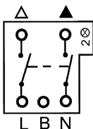
Kobling 2 2 polet
