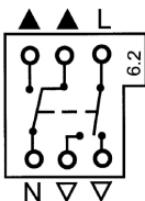
Kobling 6.2 2 Polet- Vekselvender
