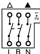
Kobling 2-1 2 Polet + 1 Polet
