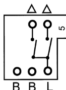
Kobling 5 Serievender
