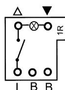
Kobling 1 R 1 Polet Imp Rele Lys
